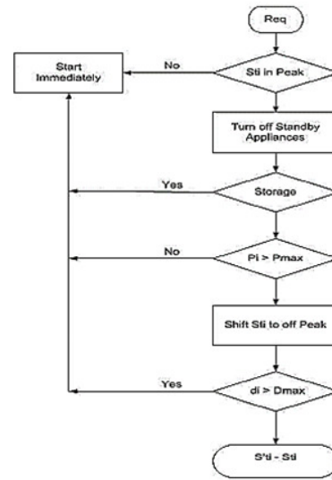
Fig. 7: HACS4EM Flowchart
